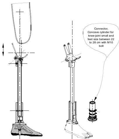
Knee-disarticulation setup
