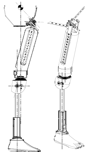
Hip-disarticulation setup
